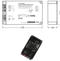
Specificaties Osram Optotronic LED Driver OT 165/170-240/1A0 4DIMLT2 G2 CE
